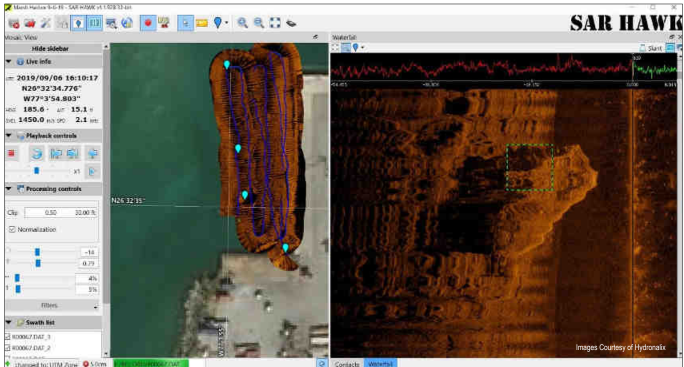
Quay wall for ship docking mapped by EMILY in Marsh Harbor, Abaco Island, Bahamas.
